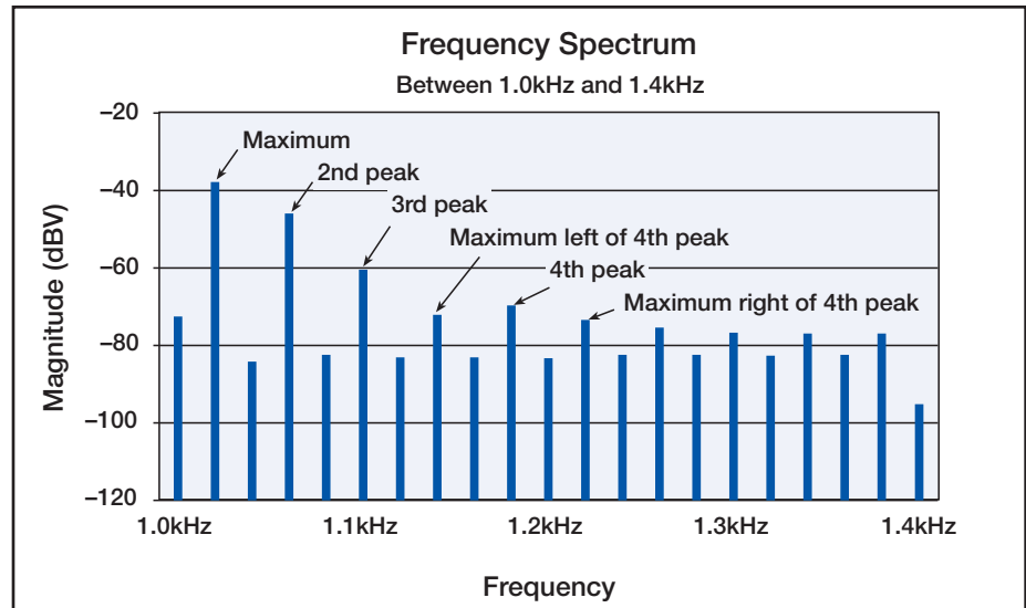
Figure 4. The Model 2015-P and 2016-P directly identify peak values of the frequency spectrum.
