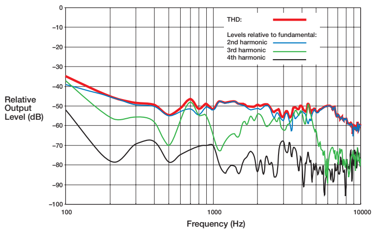
Figure 2. THD and 2nd, 3rd, and 4th Harmonics as a Function of Frequency
