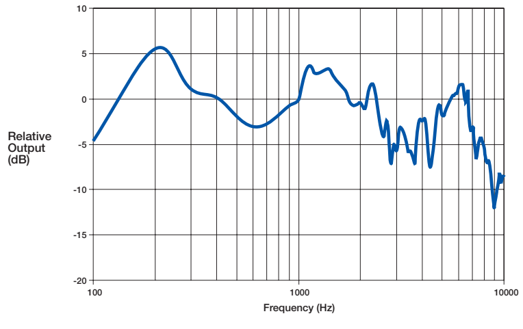
Figure 3. Frequency Response
